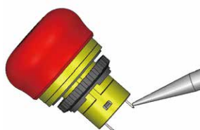
Correct
